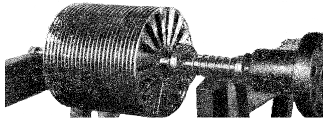
Fig. 2. Rotor of capacitive parametrical generator.
