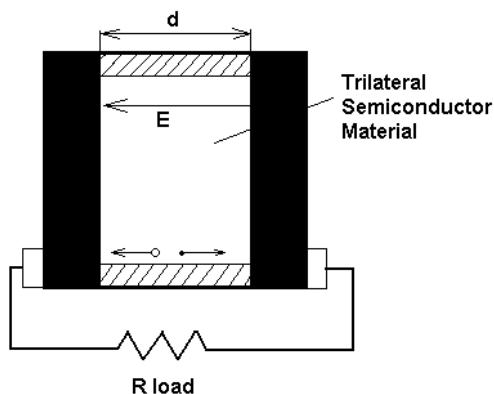
Fig. 2. Tritium Battery
