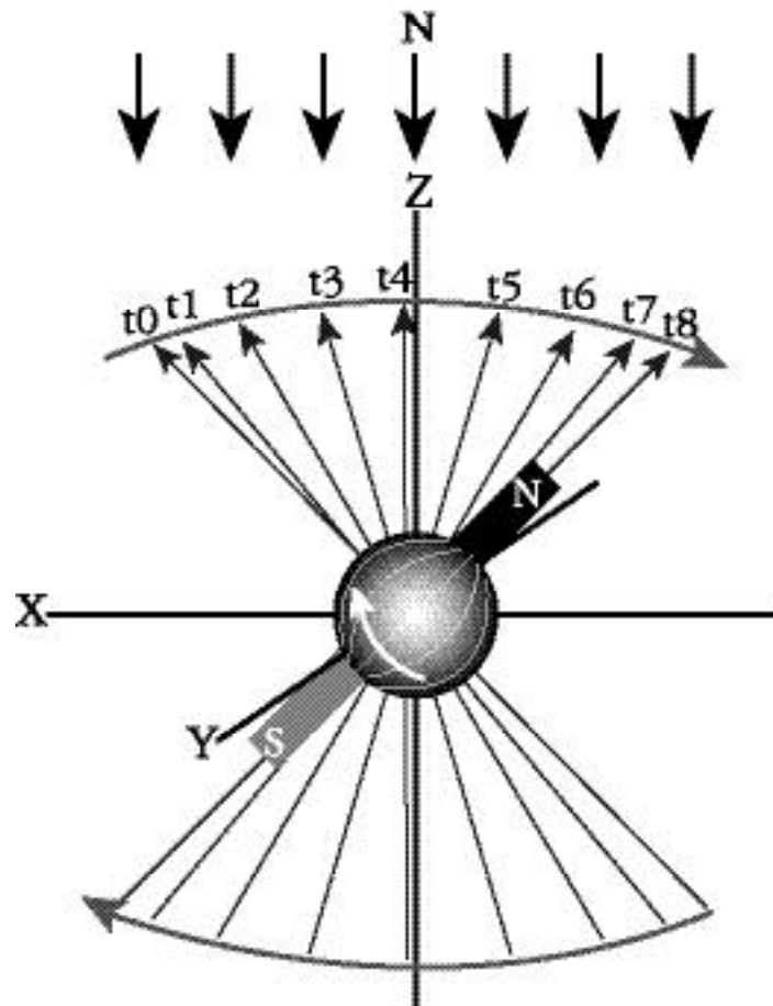
Fig. 2 Electron precession
