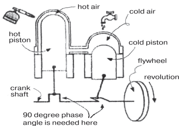
Fig. 7. External-combustion engines
