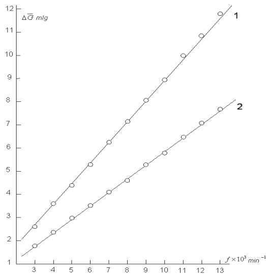
Fig. 1. 1 - rotor mass 175.504g, inertia radius 2.26cm; 2 - rotor mass 139.863g, inertia radius 1.85cm. Lines are computation; points are experiment
