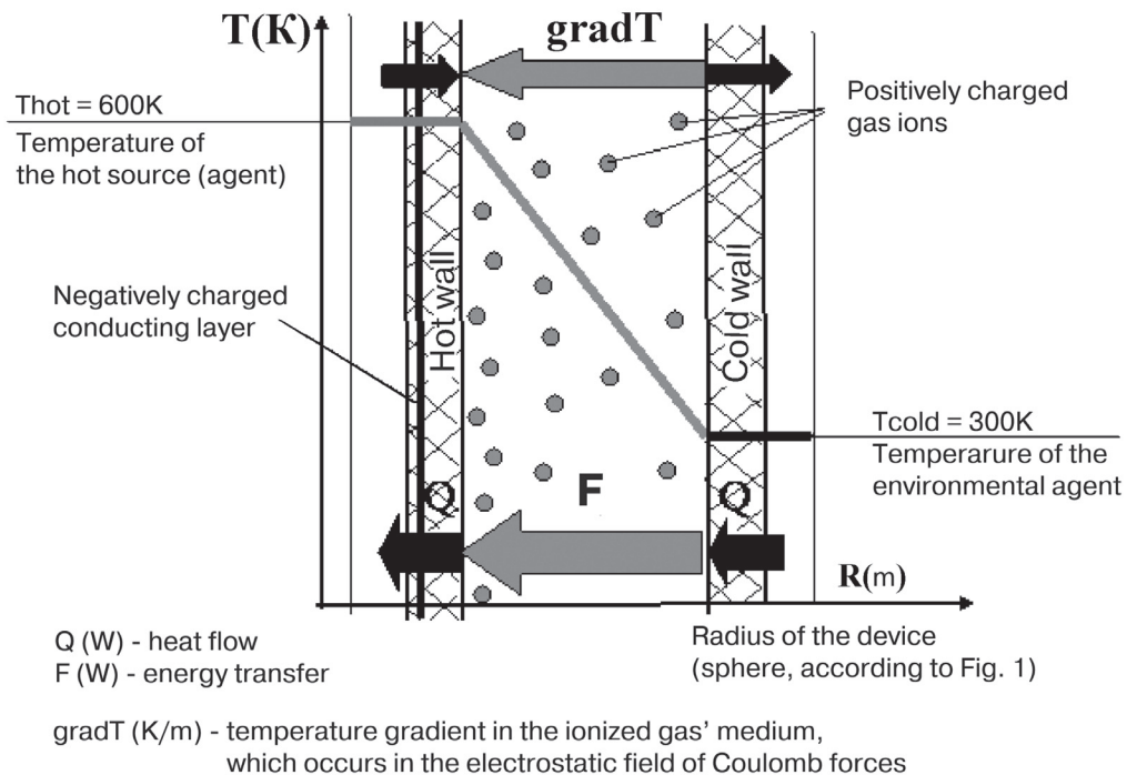
Fig. 2. Temperature field
