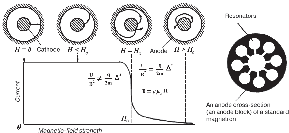
Fig. 1. Trajectories of electrons’ motion in magnetron
