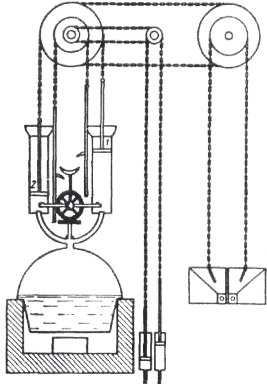
Fig. 14. I.I. Polsuniov's steamer
