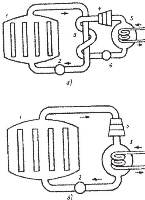
Fig. 11. Nuclear engine
