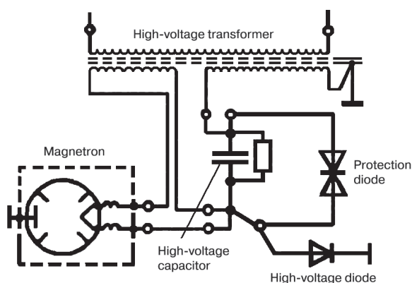
Fig. 2. Scheme of a magnetron switching on in a standard microwave oven
