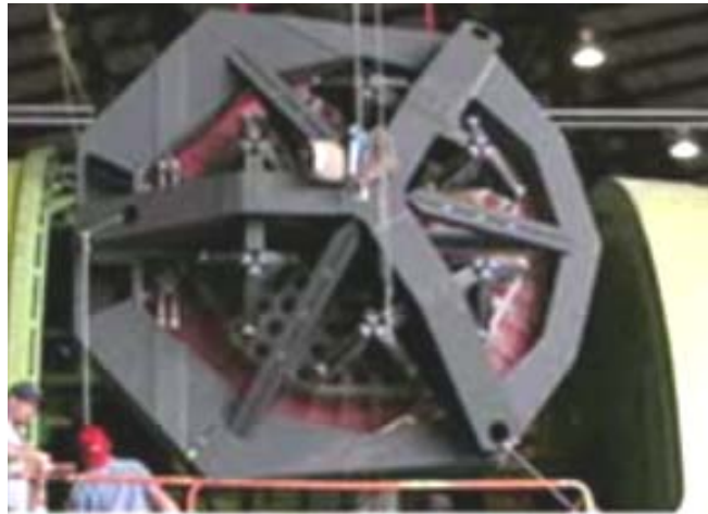
The primary mirror being lifted into the Telescope Assembly inside the plane (July 2003)
